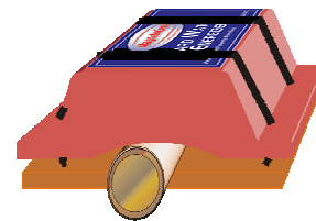
Clamp-on Unit and back plate on small copper line going into air handler
